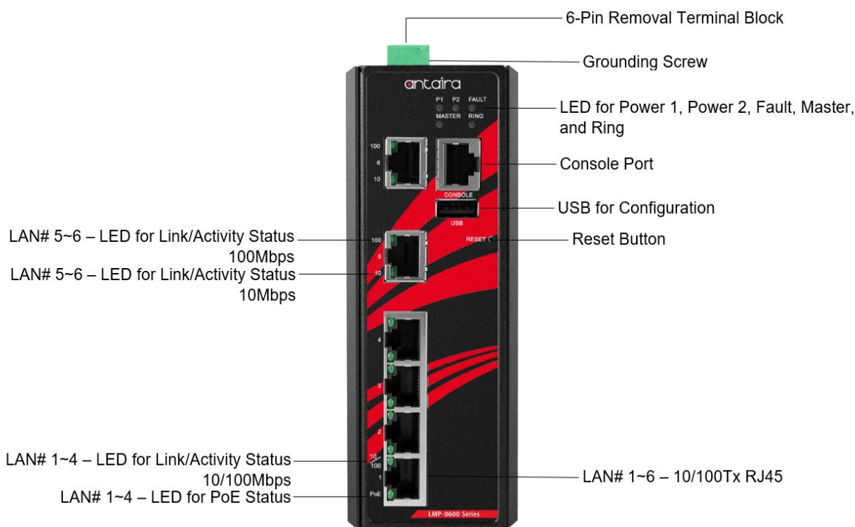
Figure 2.2 - Front View Panel
