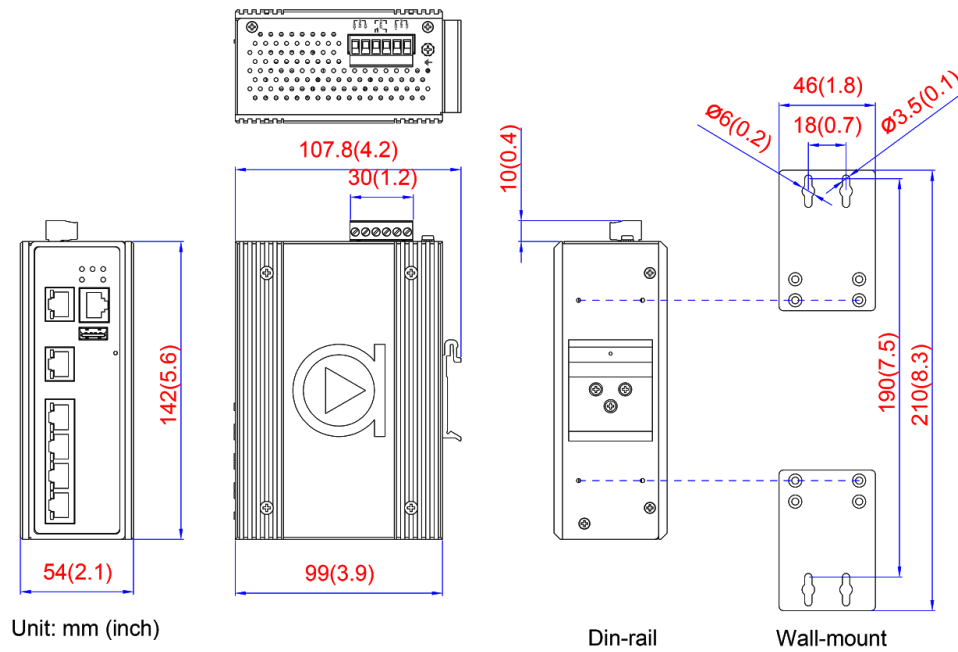
Figure 2.1 - Physical Dimensions
